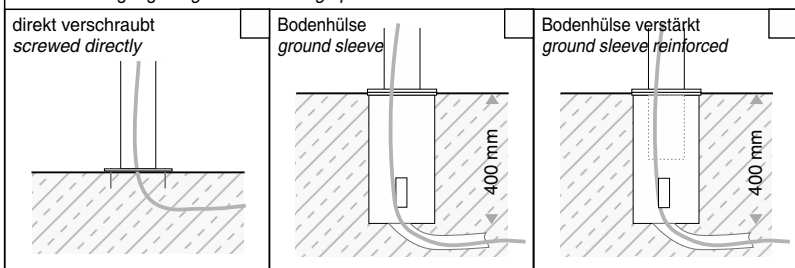
Bodenbefestigungen / ground mounting options
