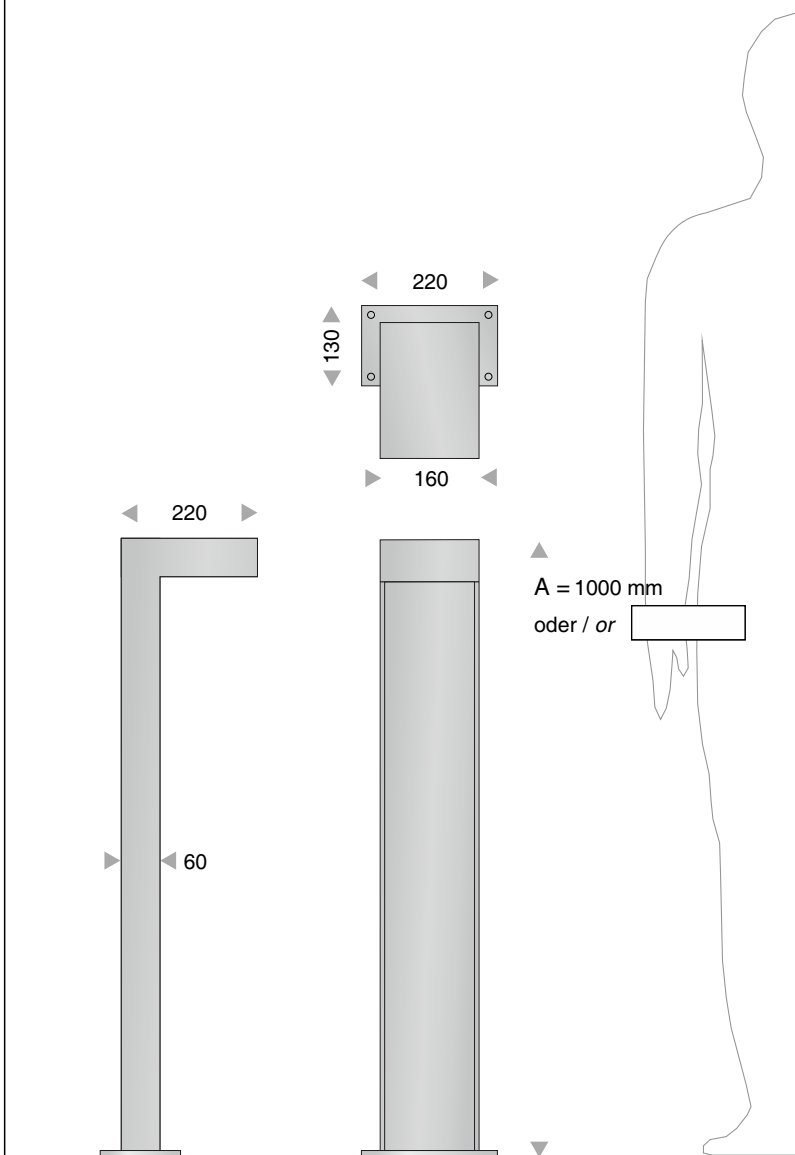
Bodenbefestigungen / ground mounting options
